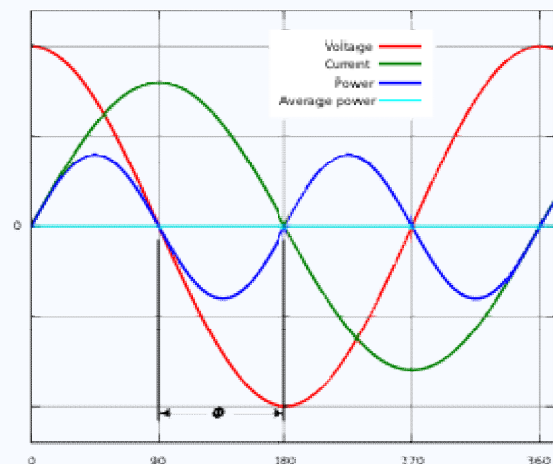
Instantaneous and average power calculated from AC voltage and current with a zero power factor ( \phi=90 , \cos\phi=0 )
