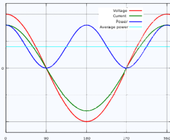
Instantaneous and average power calculated from AC voltage and current with a unity power factor ( \phi=0 , \cos\phi=1 )
